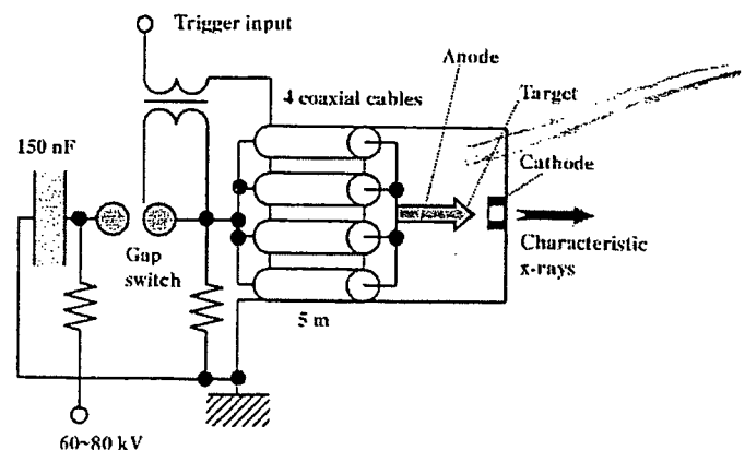
Fig. 2 Circuit diagram of the flash x-ray generator utilizing a coaxial transmission line.
