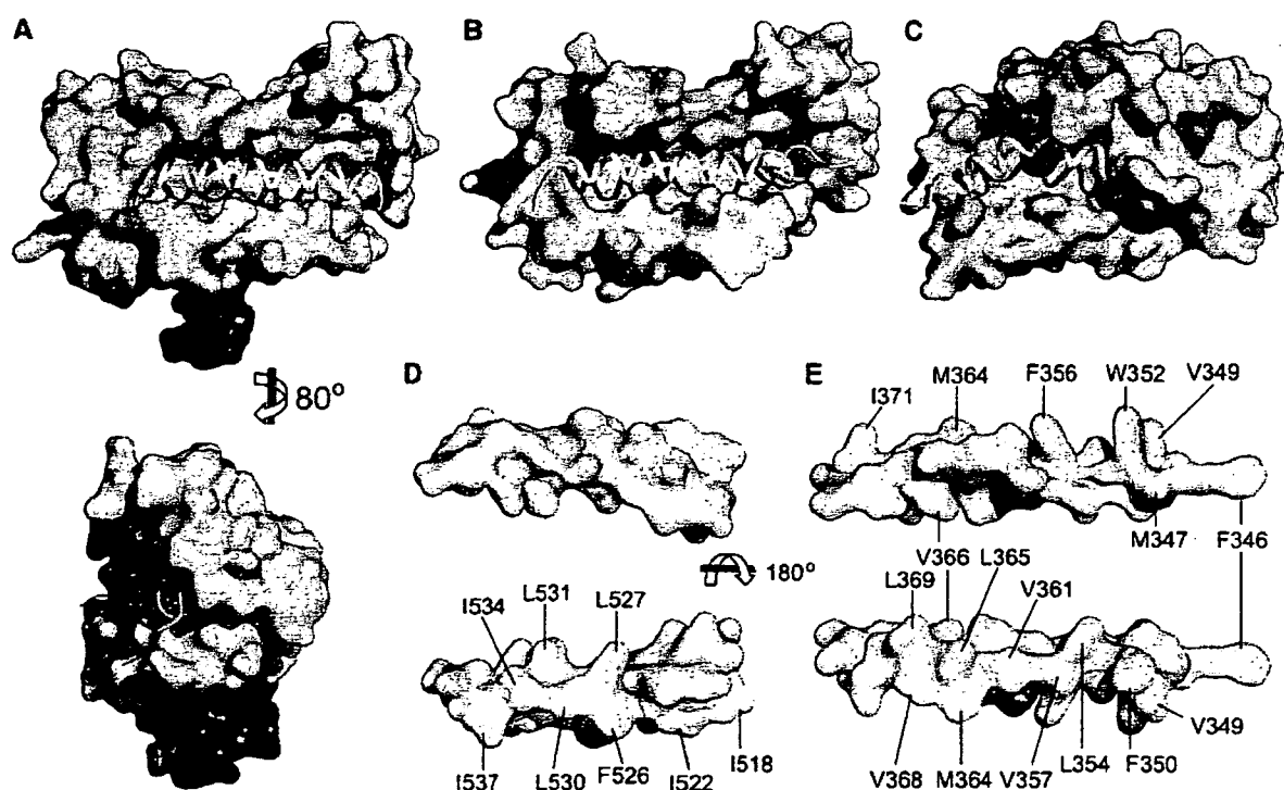
Figure 3 Target specificity of hydrophobic cleft. (A–C) Surface features of CHP2, CNB, and KChP1 are presented together with \alpha -helices of target peptides, respectively. In CHP2, front ( upper ) and side ( lower ) views are shown. The N- and C-lobes are colored light blue and light green , while the CHP-unique region is colored red . (D, E) Surface view of NHE1 ( left ) and CNA ( right ) peptides, respectively. The upper panels indicate the side facing outside the cleft and the lower panels represent the side facing the cleft. Hydrophobic residues are colored yellow .
