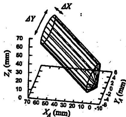
Fig. 3. Variation of position of the tip during the control of tip-rotation.
