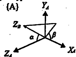
Fig. 2. Definition of positioning parameters \alpha, \beta .
