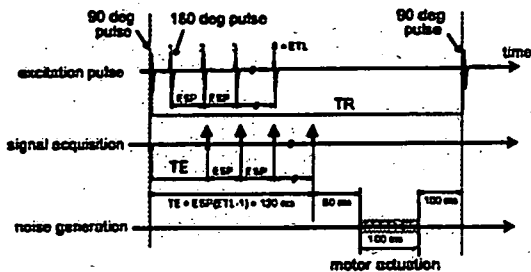
Fig. 9. Pulse sequence: experimental setting for noise evaluation.
