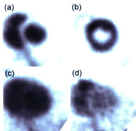
Fig. 1 Cardiac emission images for a pig with four types of tracers. (a) ^{15}\text{O} -CO, (b) ^{18}\text{F} -FDG, (c) ^{15}\text{O} -H 2 O, (d) ^{15}\text{O} -O 2 .
