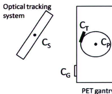
Fig. 4 Coordinates for our motion correction technique.
