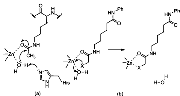
Figure 2. The mechanism proposed for the deacetylation of acetylated lysine substrate (a), and a model of the binding of heteroatom-containing substrate analogues to zinc ion (b).
