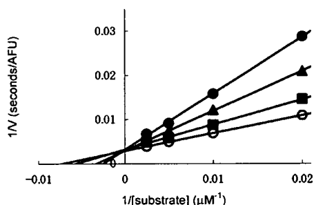
Figure 4. Reciprocal rate vs reciprocal acetylated lysine substrate concentration in the presence of 0.3 (●), 0.1 (▲), 0.03 (■), and 0 (○) \mu\text{M} of 7 .
