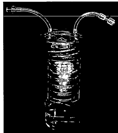
Fig. 4 Disposable capsules for hypoxic tissue culture A maximum of 5 culture dishes (6.0-cm diameter) can be placed on the tray on the stainless steel stand. The gas buffer solution is placed at the bottom of the stand. The 2 tubes protruding from the cap are the gas inlet and outlet.
