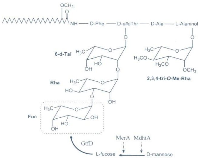
FIG. 6. Proposed structure and biosynthetic pathway of fucosylated GPL (GPL-S2).
