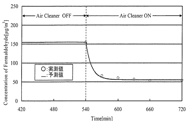
図-3 5 Formaldehyde 濃度実測値と濃度予測値との比較 (5th)
