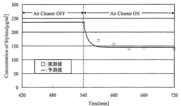
図-4 8 m-Xylene濃度実測値と濃度予測値との比較 (6th)
