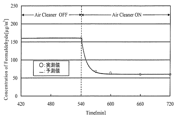
図-3 6 Formaldehyde 濃度実測値と濃度予測値との比較 (6th)
