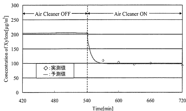
図-4 4 Styrene濃度実測値と濃度予測値との比較 (5th)
