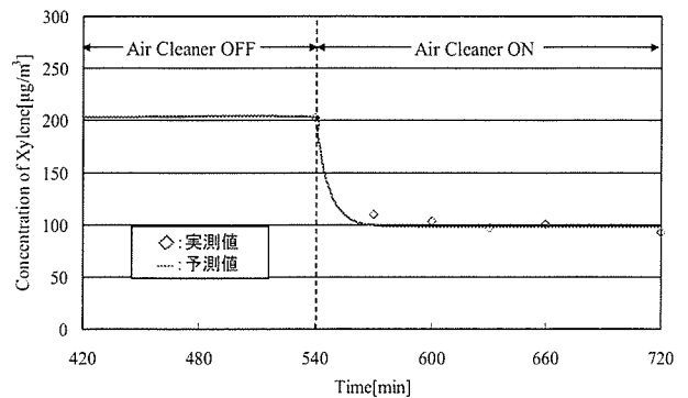
図-4 7 Styrene濃度実測値と濃度予測値との比較 (6th)
