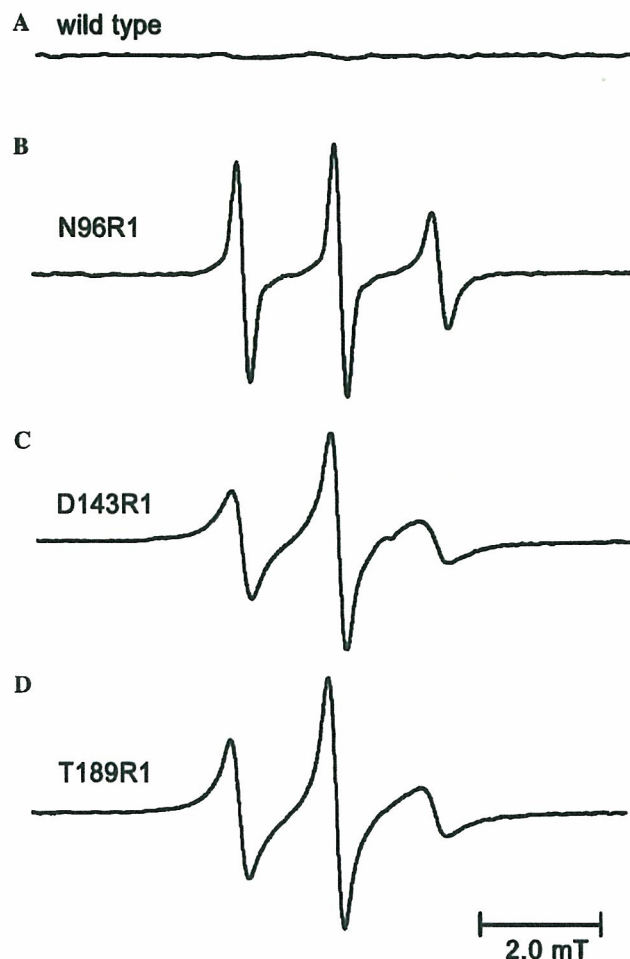
Fig. 3. X-band ESR spectra of spin-labeled recombinant moPrP mutants. After reaction of MTSSL with moPrP (wild-type) (A), moPrP (N96C) (B), moPrP (D143C) (C), and moPrP (T189C) (D), the free spin labeling compound was removed by dialysis against 10 mM acetate buffer (pH 4.0) for 48 h. pH of the sample was adjusted to 7.4 by dialysis against 10 mM Tris–HCl buffer for 4 h. ESR spectra were recorded by an X-band ESR spectrometer with a field modulation of 0.2 mT, operating at 100 kHz, an incident microwave power of 5 mW and a field sweep of 10 mT.
