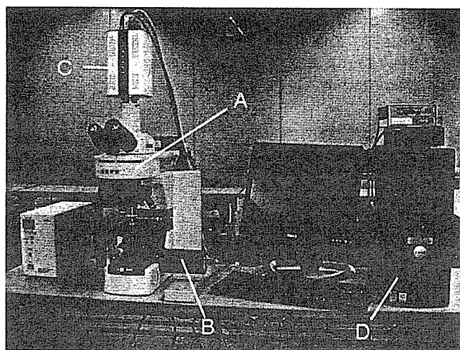
Fig. 1 UDF fluorescent microscope. A microscope, B Z-axis auto tuning system, C image detection device and D computer
