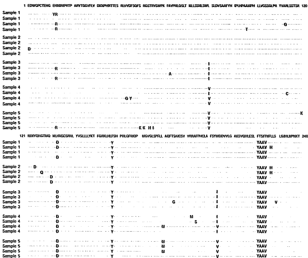
Figure 3 Comparison of amino acid sequences of HBV polymerase gene of isolates before lamivudine treatment (sample 1) and four sequential isolates (samples 2-5) during treatment. A HBV mutant with substitutions of isoleucine for leucine at residue 80 (rtL80I) in combination with isoleucine for methionine at residue 204 (rtM204I) was observed 12 mo after treatment (sample 3). After vidarabine treatment, another HBV mutant with substitutions of valine for leucine at residue 80 (rtL80V) and valine for methionine at residue 204 (rtM204V) was observed (sample 4). These mutations predominated in combination with methionine for leucine at residue 180 (rtL180M) after interferon treatment (sample 5). The published HBV DNA sequence of hepatitis B virus variant (genotype C, AB033550, Okamoto et al. 25 ) was used for comparison.
