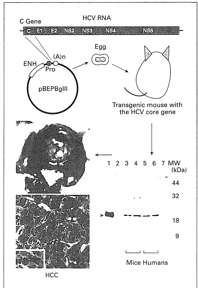
Fig. 1. Expression of HCV core gene in transgenic mouse. It carries the core gene of HCV genotype 1b alone and expresses the core protein of expected size in the liver, at levels similar to those in human patients. Mice eventually develop HCC later in their lives.
