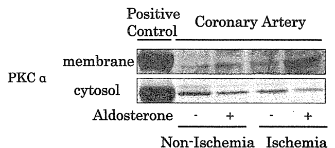
Figure 3. Effects of aldosterone on PKC \alpha activation in coronary arteries. The representative cases in Western blotting against PKC \alpha in the vascular tissues from the LAD.
