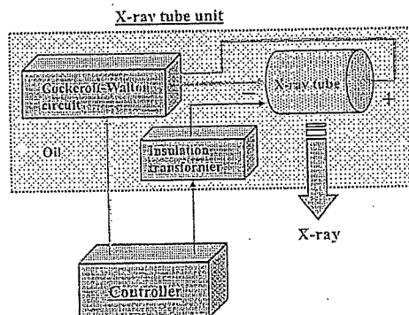
Fig. 1. Block diagram of the x-ray generator.
