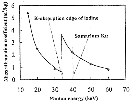
Fig. 6. Mass attenuation coefficients of iodine and average photon energy of samarium Kα lines.
