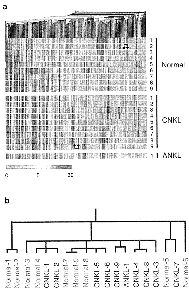
Figure 2 Expression profiles of 6494 genes in NK cell fractions. (a) Hierarchical clustering of 6494 genes on the basis of their expression profiles in CD3 + CD56 + fractions derived from nine healthy volunteers (Normal), nine individuals with CNKL, and one with ANKL. Each column represents a single gene on the microarray, and each row a separate patient sample. Expression level of each gene is shown color-coded, as indicated by the scale at the bottom. Arrows indicate the positions of clusters of genes that were expressed preferentially in either normal or affected NK cells. (b) Two-way clustering analysis of the healthy individuals (Normal-1–9), CNKL patients (CNKL-1–9), and the ANKL patient (ANKL-1), based on the similarities in the expression profiles of the 6494 genes demonstrated in (a).
