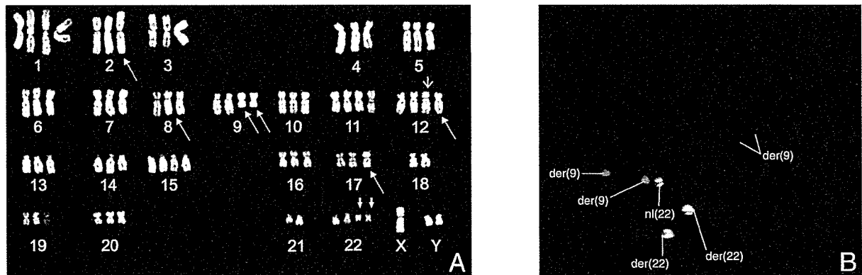
Fig. 2: Karyotype and FISH findings of TCC-S cells
