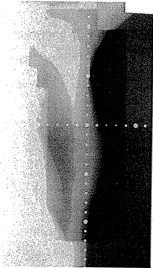
Fig 1. The irradiated field of the whole right breast with ^{60}\text{Co} \gamma rays.
