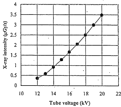
Fig. 6. X-ray intensity at 1.0 m from the pipe target according to changes in the tube voltage with a tube current of 0.10 mA.
