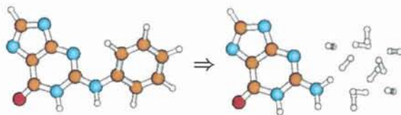
Figure 4. Structure of the H_2 cluster.
