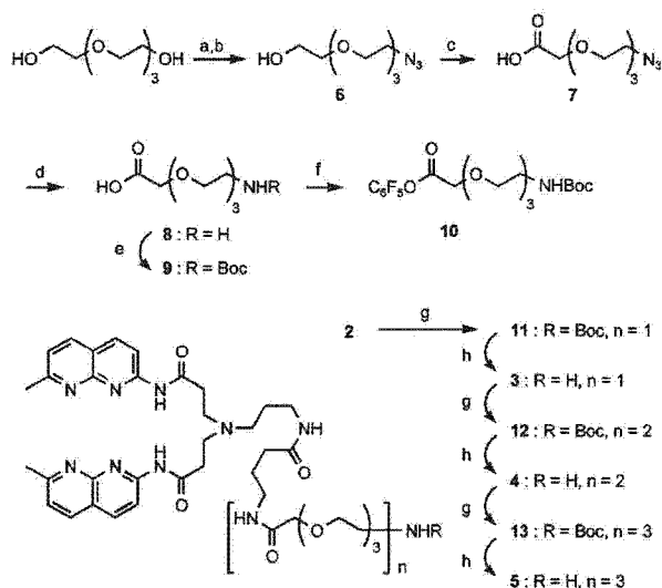
Scheme 1. Synthesis of naphthyridine dimers tethered to a different PEO linker. Reagents and conditions: (a) MsCl, NEt 3 , dry diethylether; (b) NaN 3 , EtOH, reflux, for 2 steps 46%; (c) Jones' reagent, acetone, 80%; (d) Pd–C, H 2 , EtOH, quantitative; (e) (Boc) 2 O, 2 M, NaOH, THF, 36%; (f) pentafluorophenol, EDCl, DMF, 80%; (g) 10 , Et 3 N, THF, 90% for 11 , 78% for 12 , 74% for 13 ; (h) HCl, AcOEt, CHCl 3 , quantitative.
