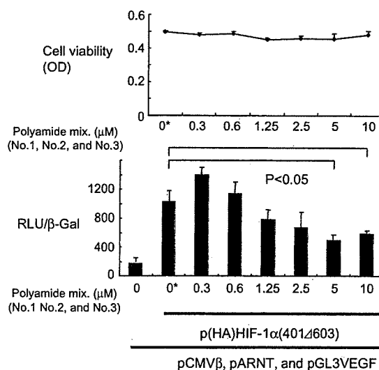
Figure 2. Dose-dependent inhibition of HIF-1 \alpha -induced transcription in 293 cells. Cells were transfected with plasmids coding hypoxia-stable HIF-1 \alpha , ARNT, and \beta -galactosidase, along with a reporter plasmid (pGL3VEGF), and then treated with the mixture of three pyrrole-imidazole hairpin polyamides for 24 h. Transcriptional activity was measured and expressed as a ratio of luciferase to \beta -galactosidase activity. Statistically significant suppression of transcription was noted at a concentration of 5 \mu M or greater. Cell viability was not affected by the polyamides. RLU and \beta -Gal denote relative luciferase units and \beta -galactosidase activity, respectively. OD: optical density. *: Vehicle (dimethylsulfoxide) only.
