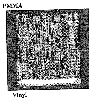
Figure 9: Radiograms of tungsten wires coiled around a rod made of polymethyl methacrylate.
