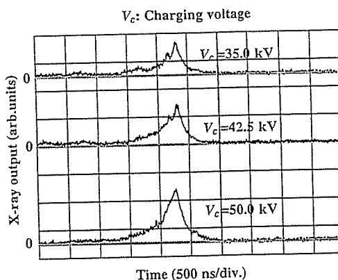
Fig. 4. X-ray outputs at the indicated conditions.
