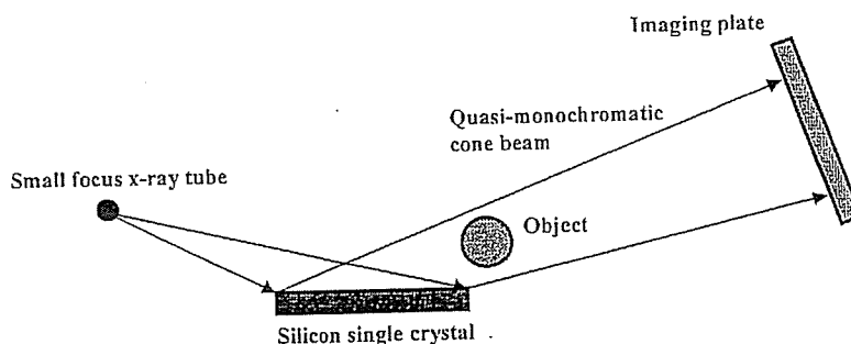
Fig. 3. Experimental setup of the narrow-photon-energy X-ray generator utilizing a single silicon crystal.
