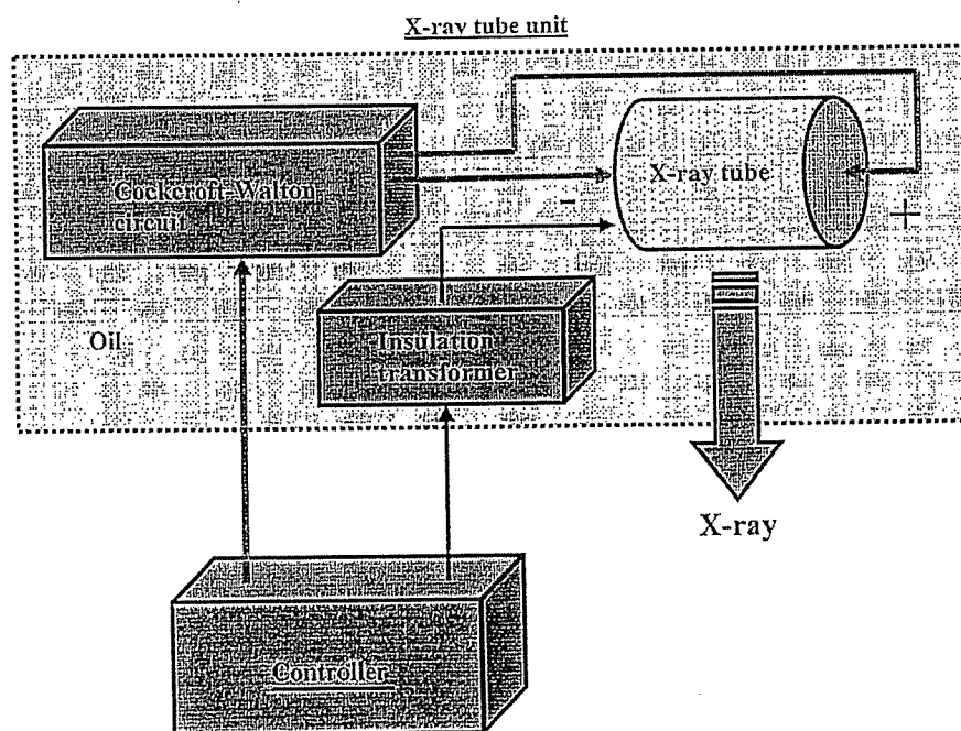
Fig. 1. Block diagram of a compact 100- \mu\text{m} focus X-ray generator with a tungsten-target radiation tube.
