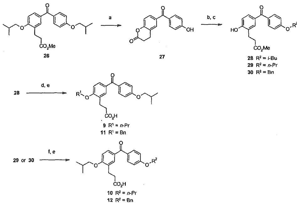
Scheme 6 a
