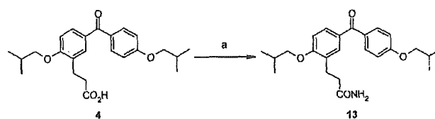
Scheme 6 a
