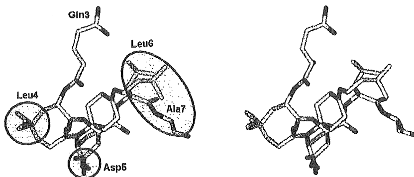
Figure 5. Stereoview of the superposition of Leu-Asp-Leu-Ala of peptide 1 (yellow) with compound 2 (white). The fitted points are shown as magenta-colored circles and an ellipse. Hydrogen atoms are not shown for clarity.
