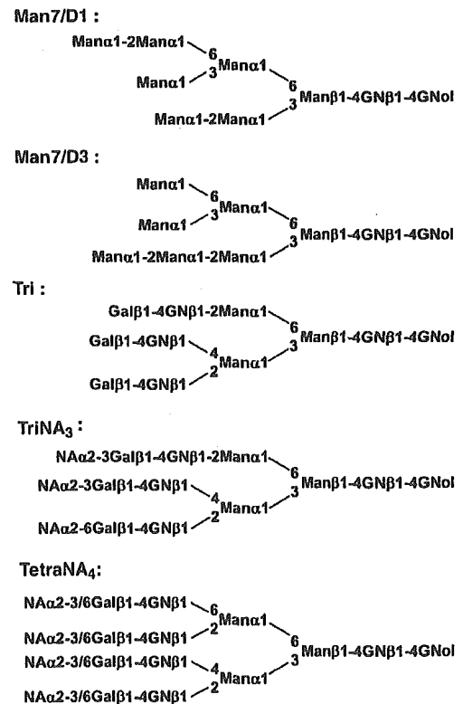
Fig. 1. Structures of major oligosaccharides and their abbreviations. Man: mannose, Gal: galactose, GN: N -acetylglucosamine, GNol: N -acetylglucosaminol, NA: N -acetylneuramic acid.
