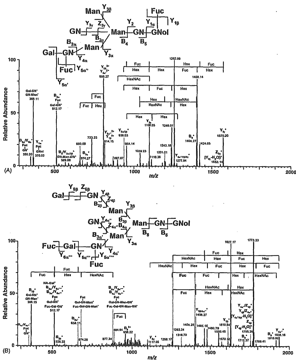
Fig. 6. Product ion spectra of N-linked oligosaccharides of rat brain Thy-1. (A) MS^2 spectrum of dHex_2Hex_4HcHexNAc_3HexNAcol_1 at m/z 887 (24.3 min). (B) MS^2 spectrum of dHex_2Hex_5HexNAc_4HexNAcol_1 at m/z 1070 (9.2 min).
