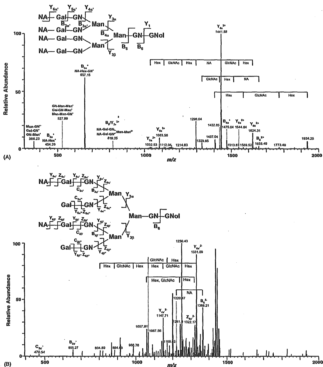
Fig. 4. Product ion spectra of model oligosaccharide, TetraNA 4 . (A) MS 2 spectrum derived from [TetraNA 4 ] 3+ at m/z 1180 in positive ion mode. (B) MS 1 spectrum derived from [TetraNA 4 ] 3- at m/z 1178 → [TetraNA 3 ] 3- at m/z 1081 → [TetraNA 2 ] 2- at m/z 1476 in negative ion mode.
