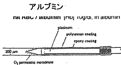
Polarographic酸素電極
