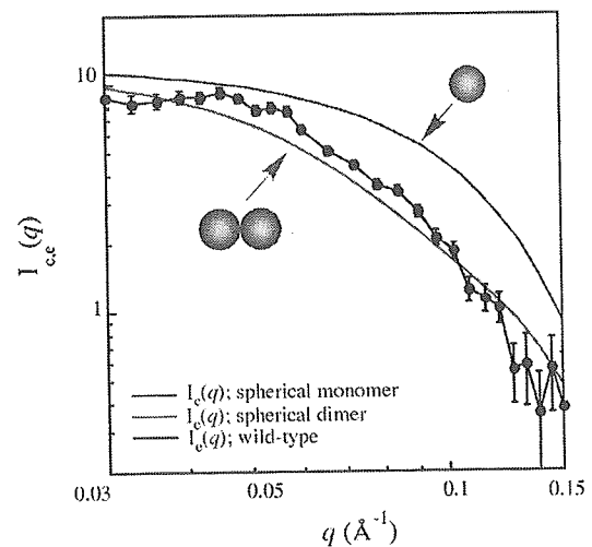
Fig. 2. The relative neutron scattering intensity ( I(q) ) versus the magnitude of the scattering vector q . I_c(q) for the wild-type UCH-L1 (black closed circle). The blue line indicates theoretical curves; I_c(q) , monomeric sphere (diameter = 21.5 Å calculated from Eq. (3), based on the R ( R = \sqrt{5/3}Rg ) value obtained using CRYSON program by Svergun [29,30]). The red line indicates theoretical curves; I_c(q) , dimeric spheres (calculated from Eq. (2), based on the distance between the center of the two particles being 43 Å).
