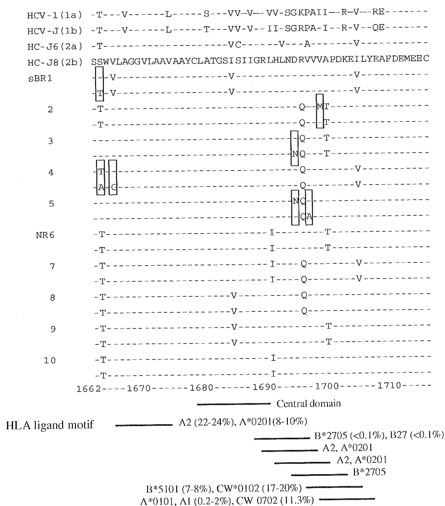
Fig. 4 Comparison of the amino acid sequences in NS4A before and after interferon (IFN) therapy, and with HCV isolates of genotypes 1a, 1b, 2a, 2b. The amino acids changed in sBR are boxed. The central domain of NS4A directly involved in NS3-NS4A complex formation and the HLA-A2 restricted epitope postulated in amino acids 1671-1680 partially overlapping this domain of NS4A in genotype 1b are indicated by solid lines below the sequence alignment, along with potential HLA class I binding motifs identified by HLA Ligand/Motif DATABASE ( http://hlligand.ouhsc.edu/LigandDB ). Numbers in parentheses indicate the gene frequency of each HLA in the Japanese population [28,29].
