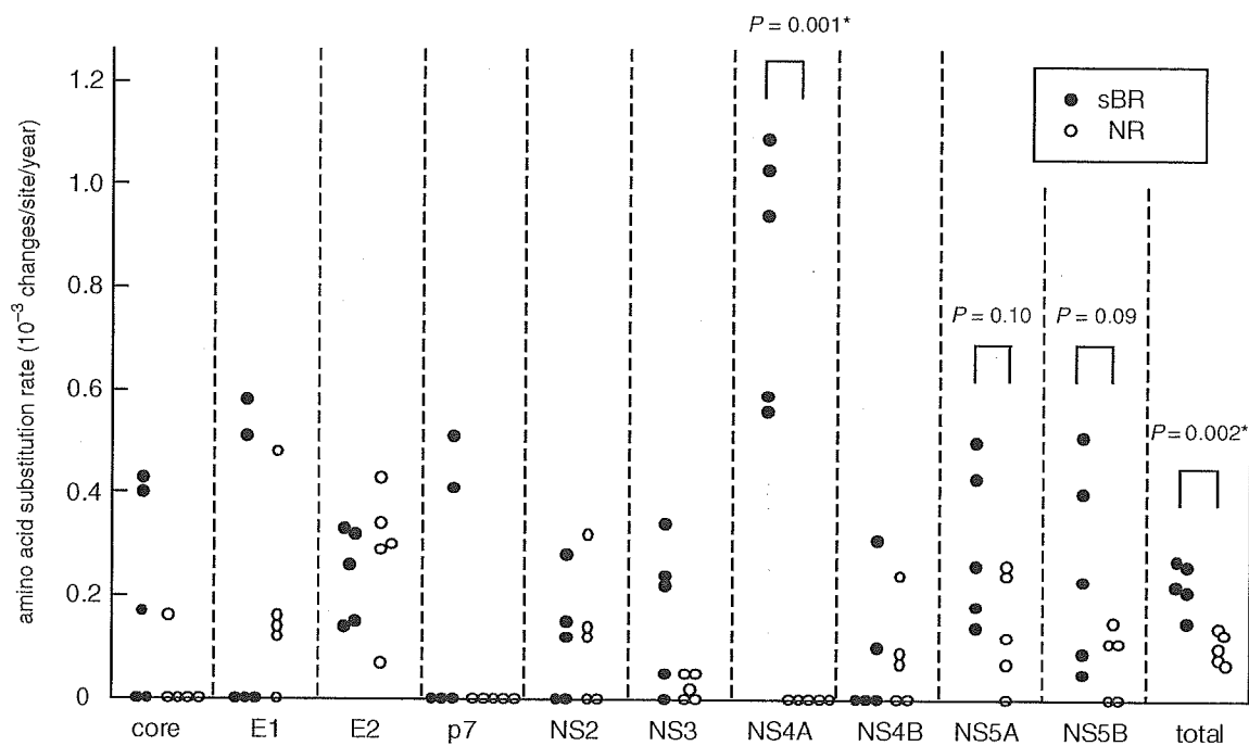
Fig. 3 The rate of amino acid substitution in each protein coding region, comparing sBR and NR groups. * P value <0.01 .
