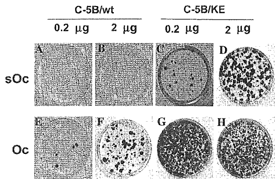
Fig. 5. Effect of K1609E on ECF. ECF was examined using cured cell lines, sOc and Oc. G418-resistant colonies were stained with Coomassie brilliant blue at 3 weeks after electroporation of RNA transcripts without (C-5B/wt; A, B, E, and F) or with (C-5B/KE; C, D, G, and H) the K1609E mutation (0.2 and 2 µg per 10-cm dish) into sOc cells (top panel) or into Oc cells (bottom panel) [22].
