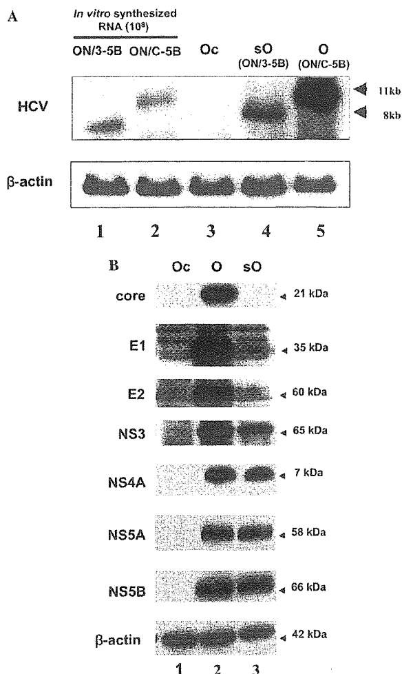
Fig. 2. Detection of HCV RNA and proteins in G418-resistant cell line. (A, top panel) Northern blot analysis of HCV-specific RNA in G418-resistant genome-length HCV RNA-replicating cell line. Lanes 1 and 2, synthetic RNA transcribed from ON/3-5B and ON/C-5B, respectively; lane 3, cured HuH-7 cells (Oc); and lanes 4 and 5, clonally isolated subgenomic HCV replicon and genome-length HCV RNA replicating cell lines by G418 selection, sO (ON/3-5B) and O (ON/C-5B), respectively. (Bottom panel) Northern blot analysis of \beta -actin mRNA using \beta -actin-specific RNA probe. (B) Western blot analysis of HCV proteins. Production of core, E1, E2, NS3, NS4A, NS5A, and NS5B in Oc cells (lane 1), O cells (lane 2), and sO cells (lane 3) was analyzed by immunoblotting using anti-core, anti-E1, anti-E2, anti-NS3, anti-NS4A, anti-NS5A, and anti-NS5B antibodies, respectively. \beta -actin was used as a control for the amount of protein loaded per lane.
