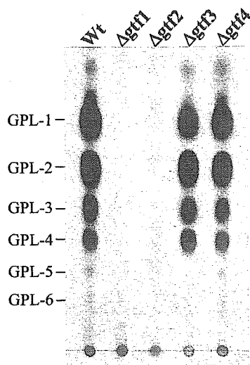
FIG. 2. TLC analyses of crude GPL extracts from the M. smegmatis mc 2 155 strain (Wt) and its gene disruptants. The total lipid fraction after mild alkaline hydrolysis was spotted on plates and developed in CHCl 3 -CH 3 OH (9:1 [vol/vol]). GPLs were visualized by spraying with 10% H 2 SO 4 and charring. Each total lipid fraction was extracted from an equal weight of harvested cells.
