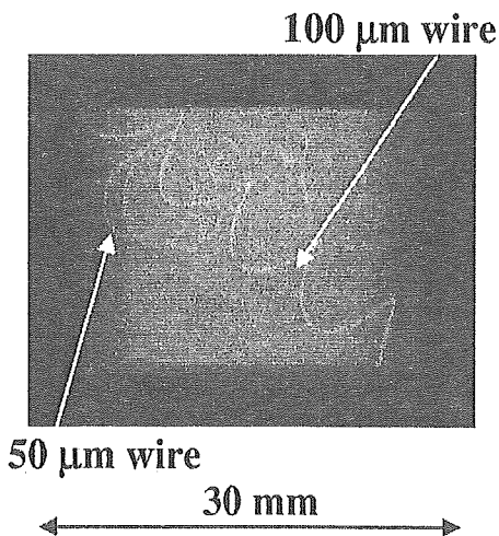
Fig. 9 Radiograms of tungsten wires of 50 and 100 μm in a rod made of polymethyl methacrylate.
