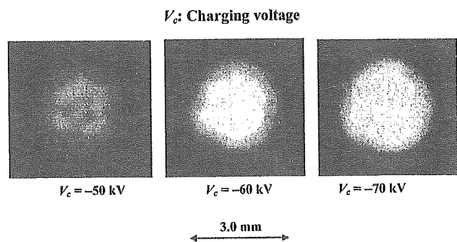
Fig. 7 Images of x-ray sources of Kα lines with changes in the charging voltage.
