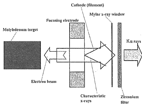
Figure 3: K-photon irradiation from the x-ray tube.
