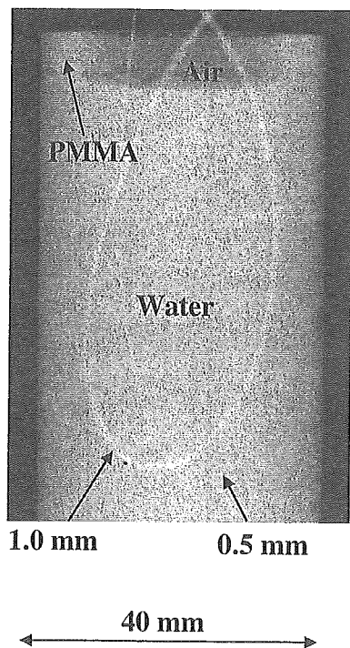
Fig. 10. Angiography of Tefflon tube using contrast medium which contains approximately 65% gadodiamidehydrate.
