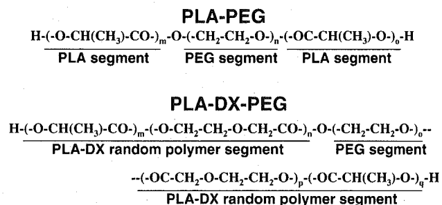
Fig. 1. Structural formulas of poly-D,L-lactic acid-polyethylene glycol block copolymer (PLA-PEG) and poly-D,L-lactic acid- p -dioxanone-polyethylene glycol block copolymer (PLA-DX-PEG). Both are A–B–A type polymers. m, n, o, p, q: number of units.
