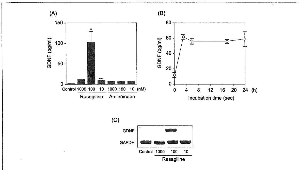
Fig. 10. Induction of GDNF synthesis and release by rasagiline in SHSY-5Y human dopamine neuroblastoma cells (ref. 146).
