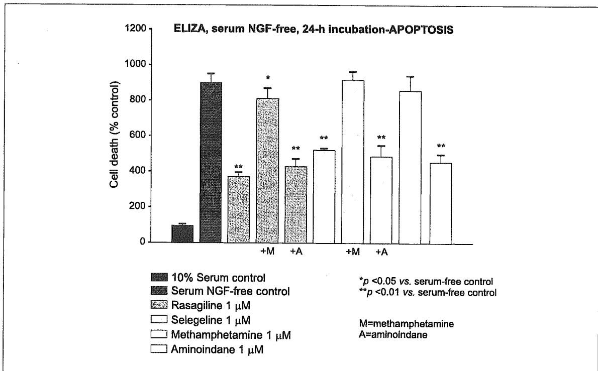
Fig. 4. The neuroprotective effect of rasagiline's metabolite aminoindane and the neurotoxicity of selegiline's metabolite methamphetamine in PC-12 cells (ref. 84).
