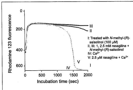
Fig. 8. Prevention of the permeability transition by rasagiline in isolated mitochondria as induced by N -methyl-( R )-salsolinol, but not of that induced by Ca^{2+} (ref. 99).
