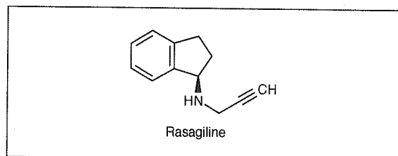
Fig. 1. The chemical structure of rasagiline.
