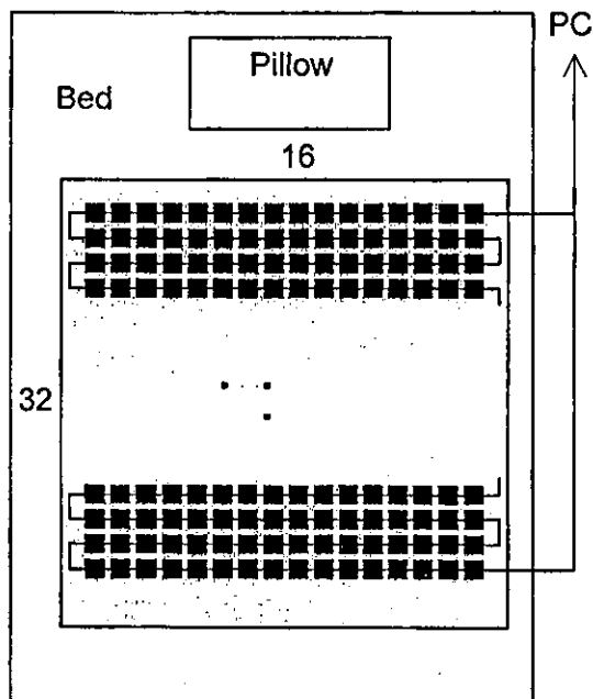
Fig. 2 Structure of Matrix Thermometer
