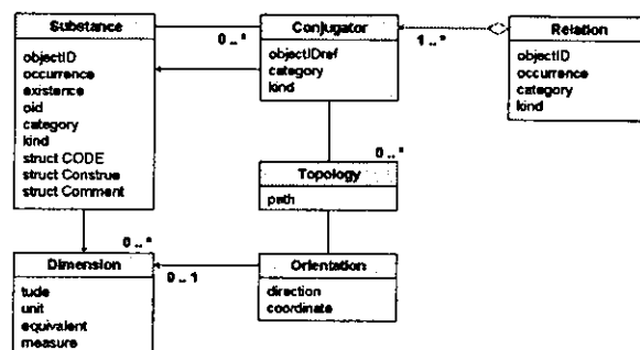
Figure 1 - class diagram
