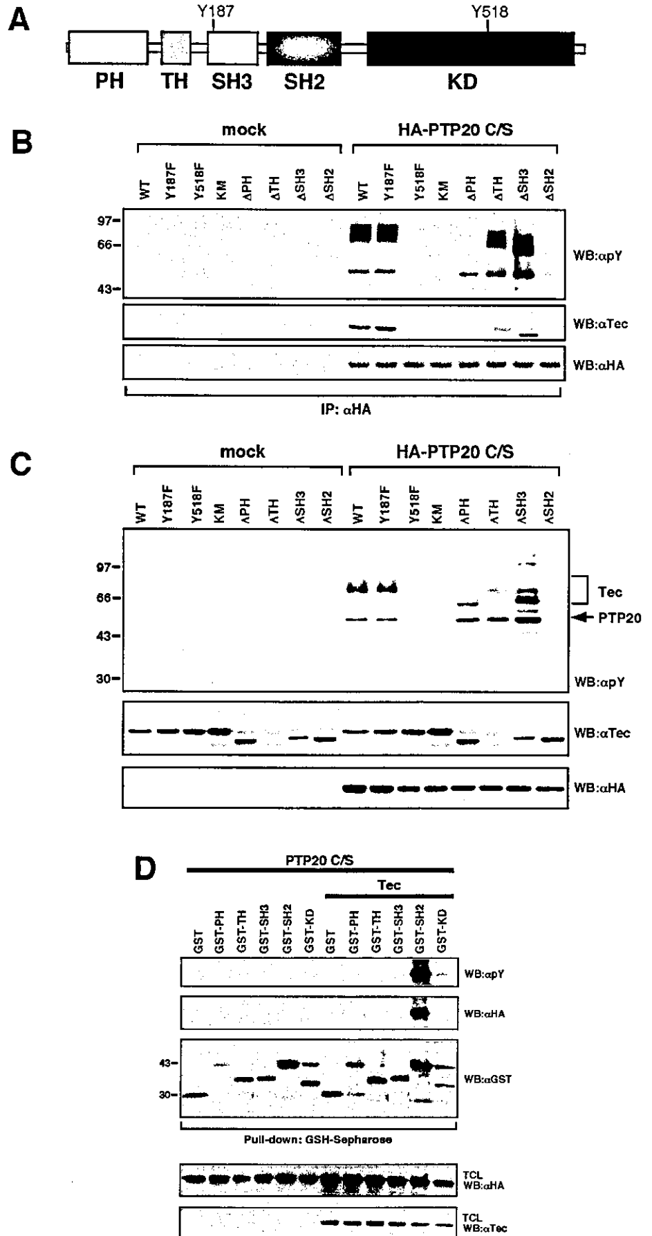
FIG. 3. Tec SH2 domain is essential for both tyrosine phosphorylation of PTP20 and association of Tec with PTP20. A , schematic organization of mouse Tec into PH, TH, SH3, SH2, and kinase ( KD ) domains. B , COS7 cells were transiently transfected with either empty vector ( mock ) or HA-PTP20 C/S together with the indicated Tec mutants. Cells were lysed, and HA-PTP20 was immunoprecipitated ( IP ) followed by immunoblotting ( IB ) with anti-phosphotyrosine antibody (PY99 ( \alpha pY)). The same membrane was sequentially reprobed with anti-Tec and anti-HA antibodies after stripping. C , aliquots of the total cell lysates ( TCL ) were separated by SDS-PAGE followed by immunoblotting with indicated antibodies. D , COS7 cells were transiently transfected with pEBG empty vector (GST) or bearing each of Tec domains (PH, TH, SH3, SH2, and KD) in the absence or presence of Tec plasmid. Cells were lysed, and GST fusion proteins were precipitated by GSH-Sepharose beads followed by immunoblot analysis with anti-phosphotyrosine ( \alpha pY) antibody. The same membrane was sequentially reprobed with indicated antibodies. Expression of PTP20 and Tec was confirmed using aliquots of total cell lysates ( TCL ) by immunoblotting as indicated.
