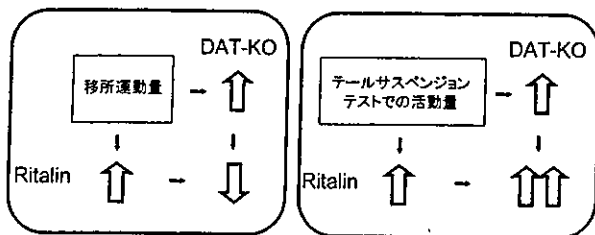
Figure 2. Opposite effects of Ritalin on mouse activity in locomotion and tail-suspension tests
