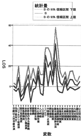
図C群 (LOS分析)
