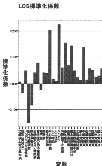
図C群 (LOS分析)
