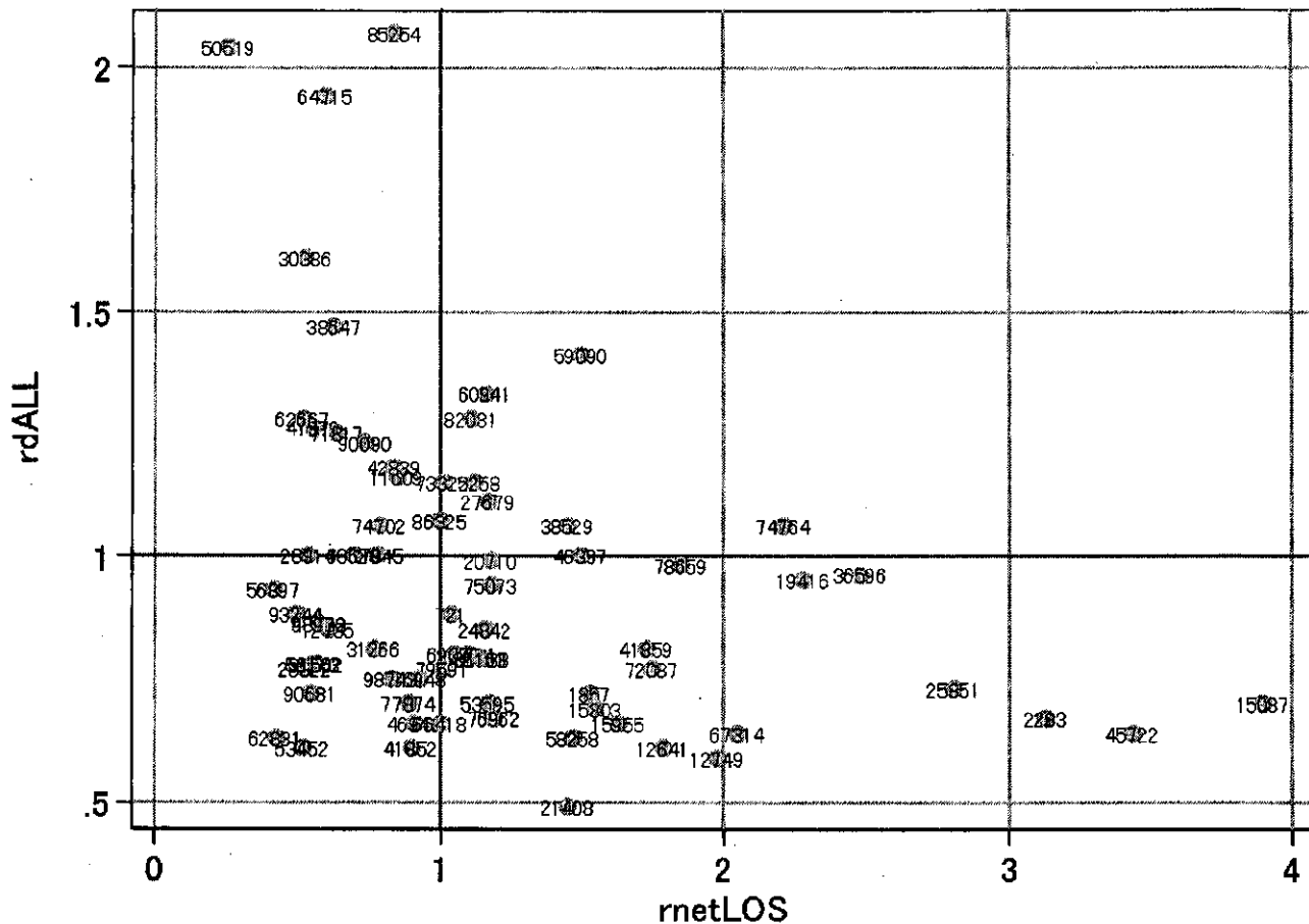
1300303x991x0x-density
