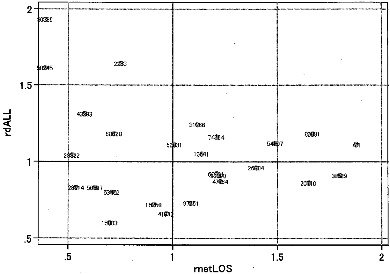
1300103x991x1x-density
