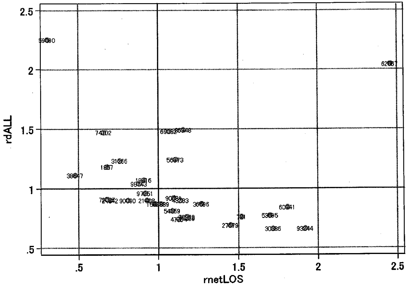
0600503x050x0x-density
