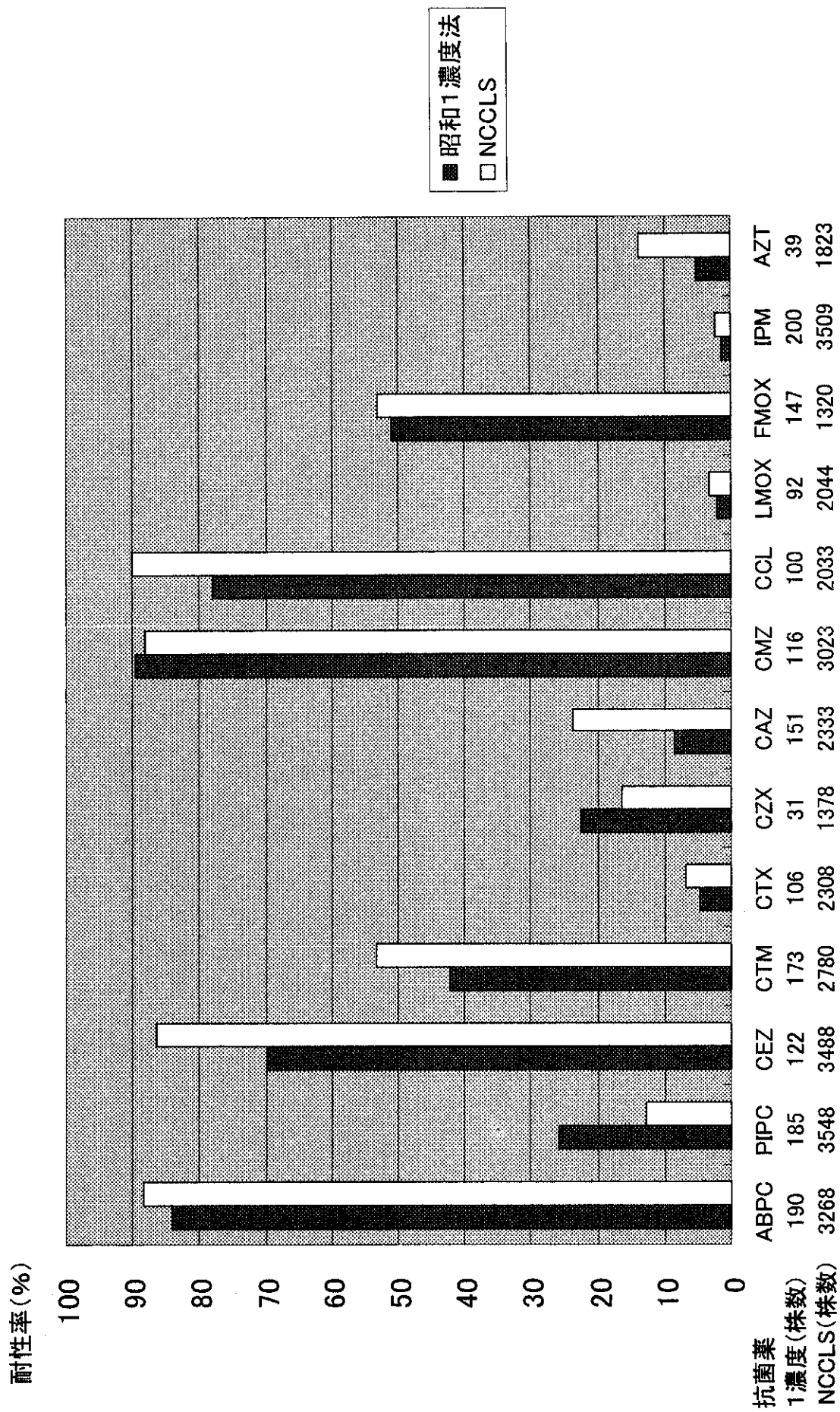
図24-1 Enterobacter aerogenes
