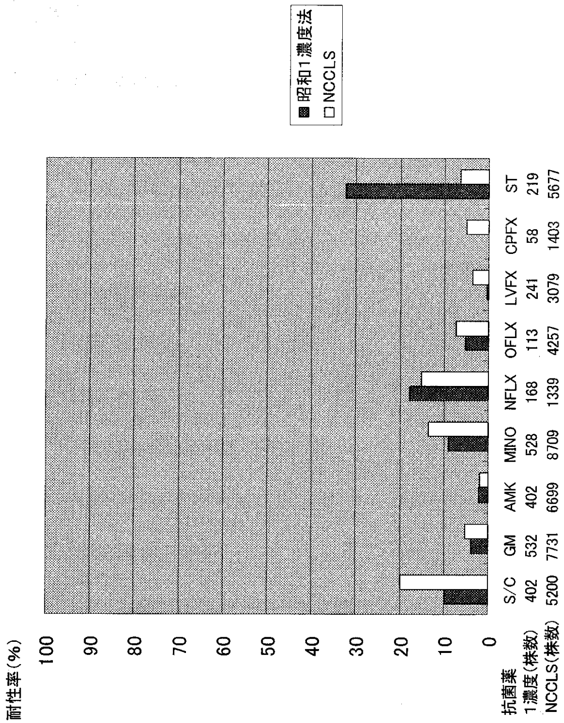
図23-2 Enterobacter cloacae
