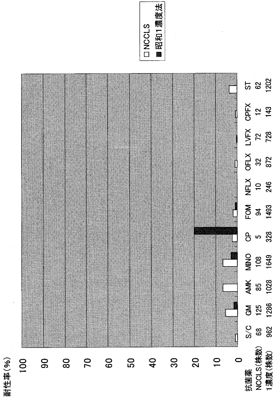
図26-2 Salmonella spp.
