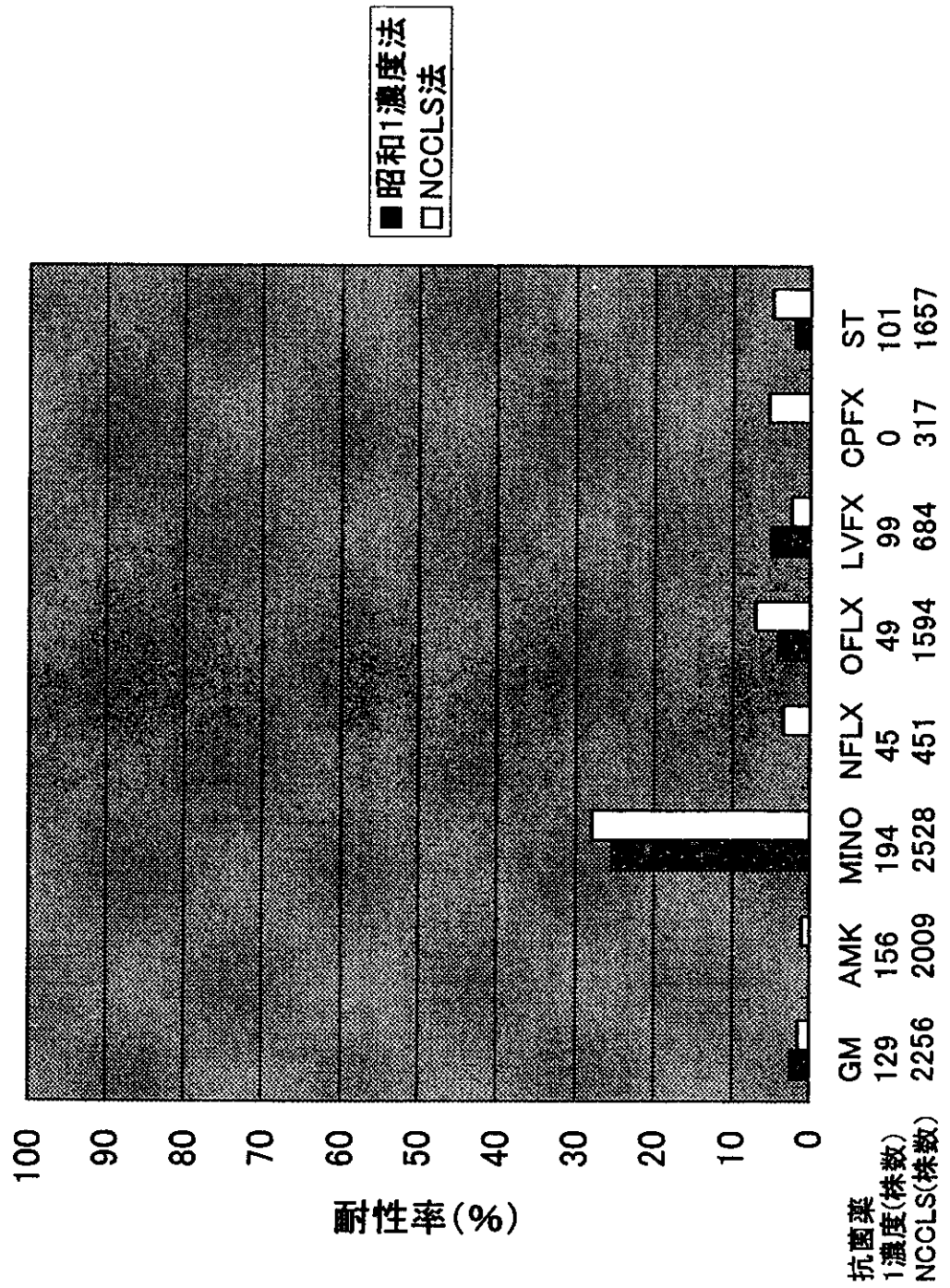
图29-2 Proteus vulgaris
